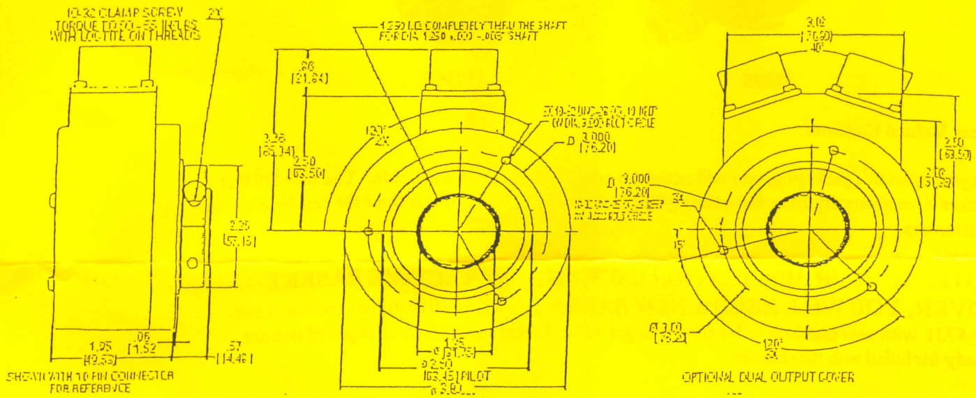
HS35R Dimensions
