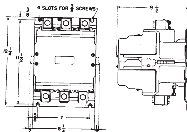
300 amp contactor
