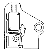
CAM FOLLOWER ACTUATOR FOR FEATURE "02" AND SPECIAL CUT OR MOLDED CAMS
