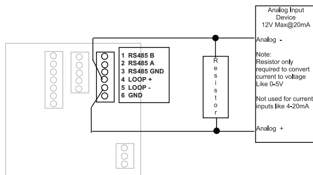
Figure 10: Current Sourcing Analog Output
