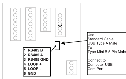
Figure 12: Analog Output Wiring
