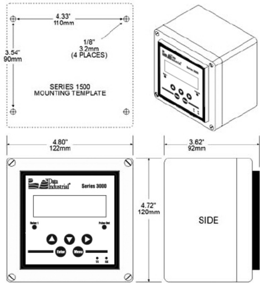
Figure 2: Wall Mount and Dimensions
