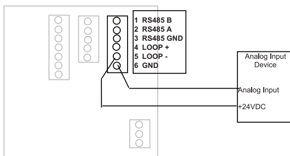
Figure 11: Current Sinking Analog Output
