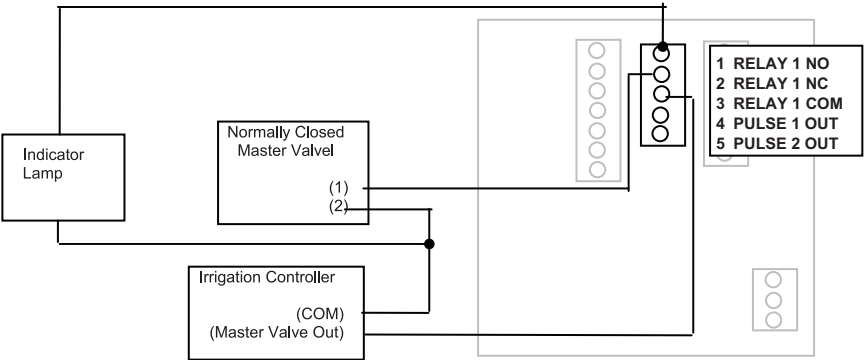
Figure 9: Relay and Switch Wiring Examples (continued) High Flow Shut Down and Irrigation Clock Normally Closed Master Valve with Indication Program as High Flow with Latch
