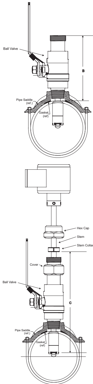
Figure 9: Sensor tip and stem collar
