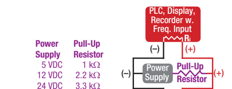
MOSFET Open Collector Output
