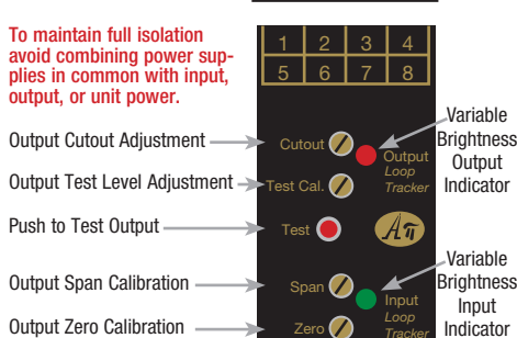
Output Cutout Adjustment
