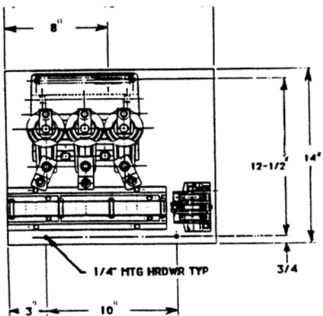
Open Starter 3.3 KV, 160-320A
