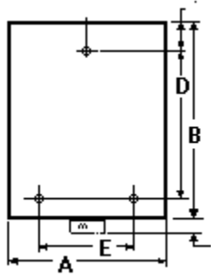
NEMA Type 1 Enclosure
