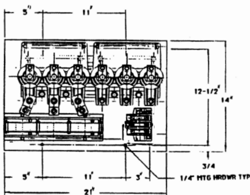
Open Starter 1.5/3.3 KV, 600A
