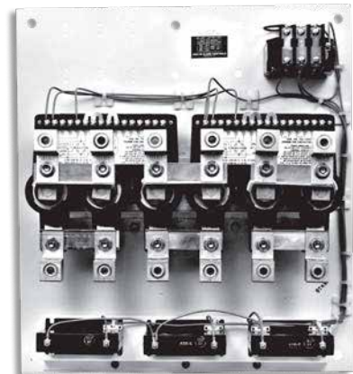
Open Type 500HP 460V 1600 HP 1500V
