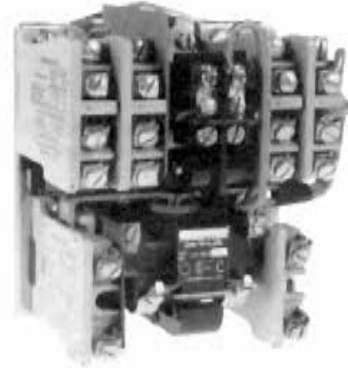
Typical 30 Ampere Electrically Held Lighting Contactor, 8-Pole
