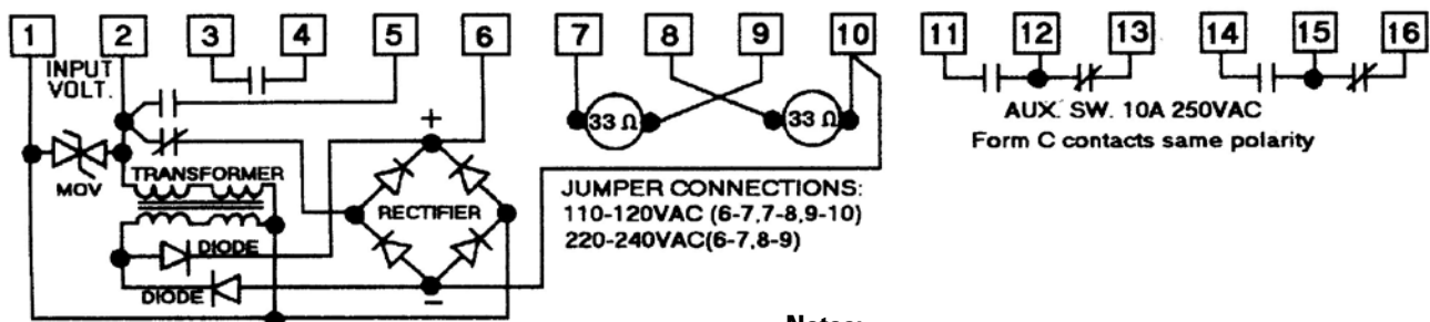
Control Diagram
