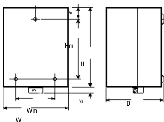
NEMA Type 1 Enclosure
