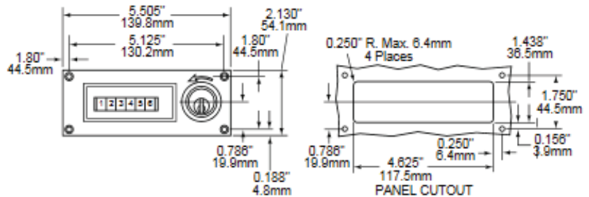
Panel Mount, Lock & Key Reset Depth: 2.530"/64.3mm
