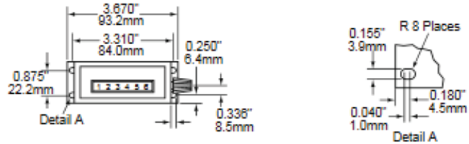
Base Mount, Knob Reset Depth: 2.570"/65.2mm
